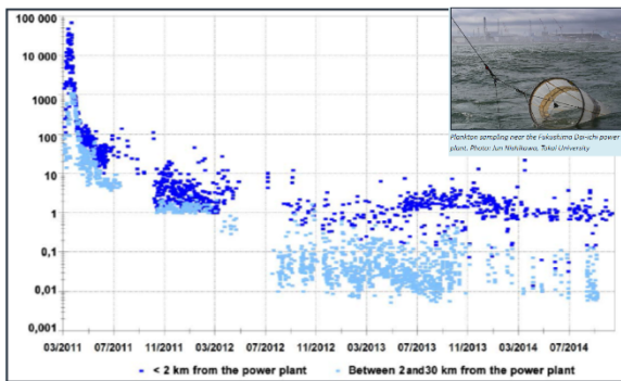
Radioactive caesium-137 (Bq/L) in seawater from 2011 to 2014. www.irsn.fr
